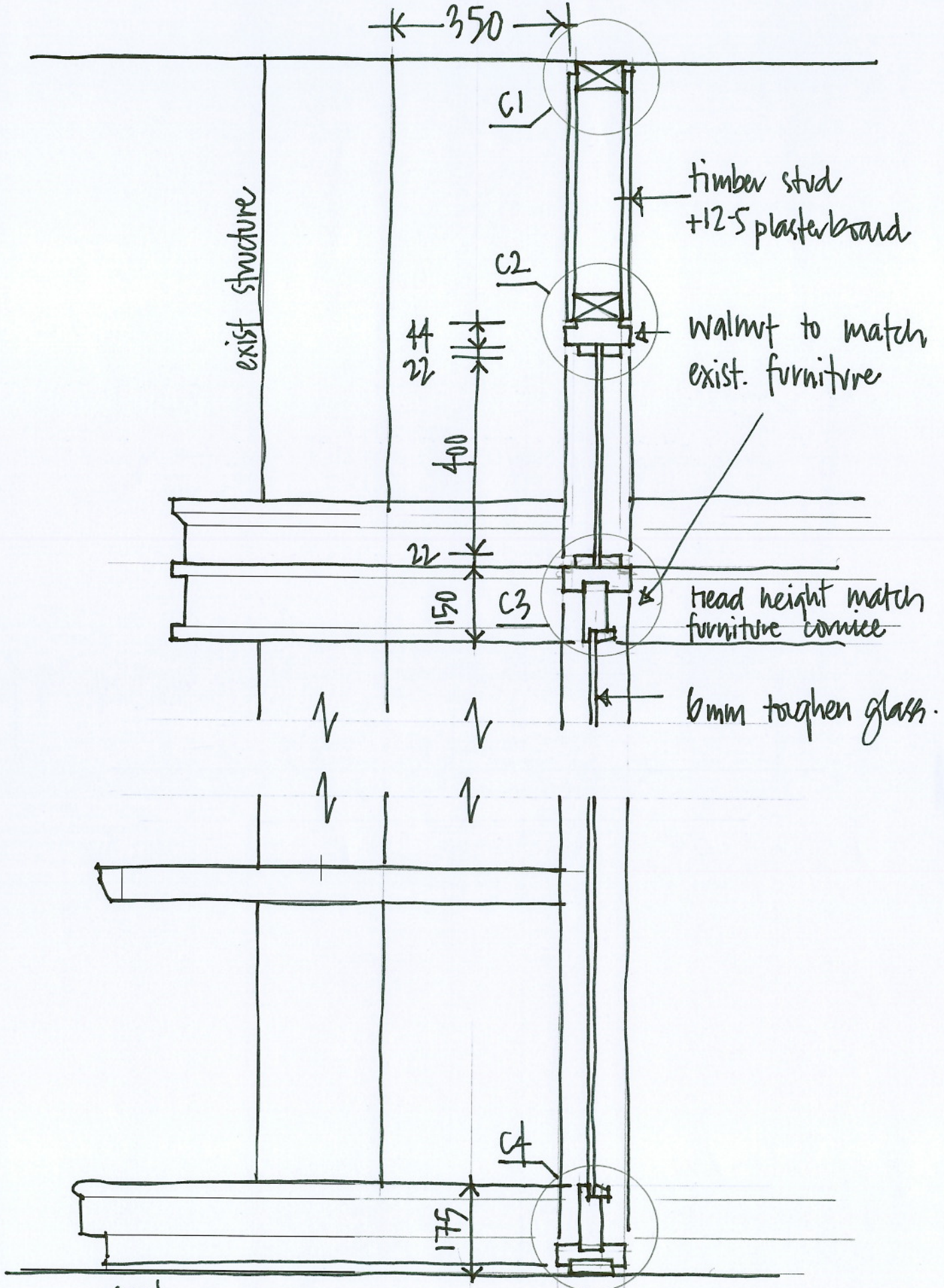
SECTION C-C
